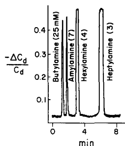
Fig. 8. A separation of four aliphatic amines with DLC detection at E = -0.45 V. Conditions: column, Bio-Rad Anion-OH guard, 3\text{ cm} \times 4.6\text{ mm} ; eluent, 0.015\text{ M} potassium hydroxide (high-purity, Alfa).
