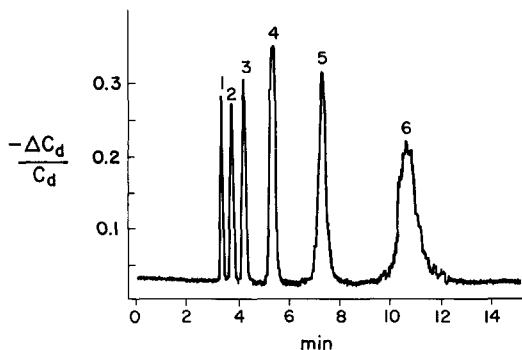
Fig. 7. Separation of six dicarboxylic acids with DLC detection; conditions as in Fig. 3 except that t_{\text{col}} = 65^\circ\text{C} and the Polypore H column was 25 cm rather than 10 cm long. Peaks: 1 = succinic (40); 2 = glutaric (12.5); 3 = adipic (5); 4 = pimelic (2.5); 5 = suberic (1.2); 6 = azelaic acid (1 mM).
