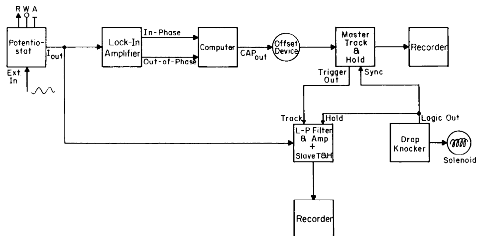
Fig. 1. Block diagram of the instrumental arrangement for double-layer capacitance detection at the DME with simultaneous faradaic electrochemical detection.
